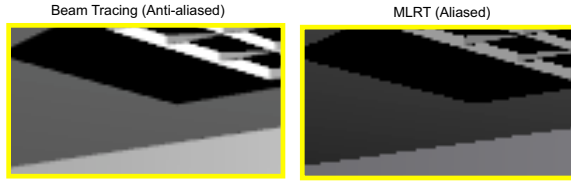
Figure 10: (Left) close-up of highlighted region from Fig. 9. We render with 6× antialiasing with almost no performance penalty. (Right) same region with MLRT clearly displaying jagged edges and spurious black pixels.
