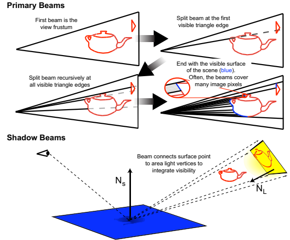
Figure 1: (Top) Beam tracing for primary visibility. (Bottom) Beam tracing for soft shadows.
