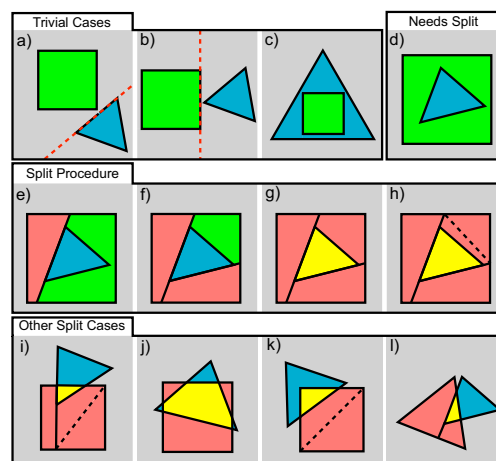
Figure 2: Illustration of beam–triangle intersection. The initial beam is green, the initial triangle is blue, miss beams are red, and hit beams are yellow. (a)–(c) are trivial cases (step 2). In (d), the beam must split (step 3). (e)–(g) split along each edge of the triangle. In (h), the beam needs an extra split to maintain a maximum of 4 vertices per beam. (i)–(l) show several other possible beam–triangle splits discussed in the text.
